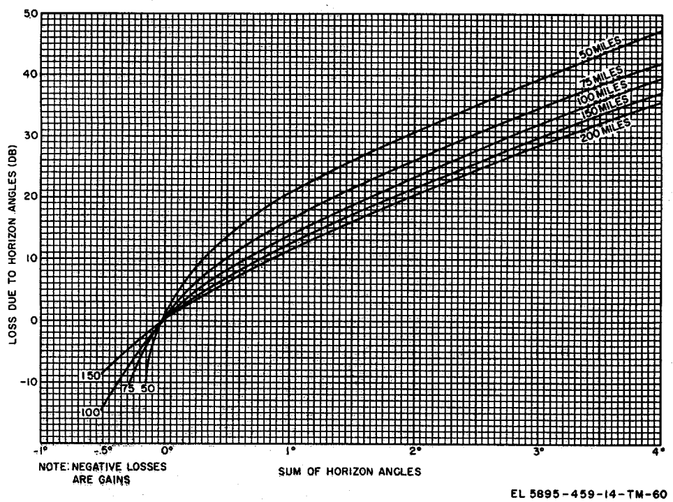
Figure 6-11. Horizon angle loss. 6-10
