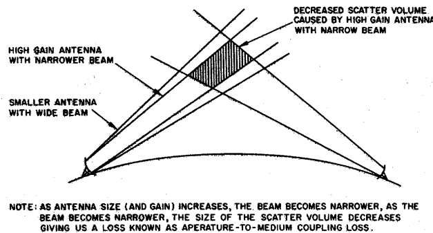
Figure 6-6. Aperture-to-medium coupling loss.
