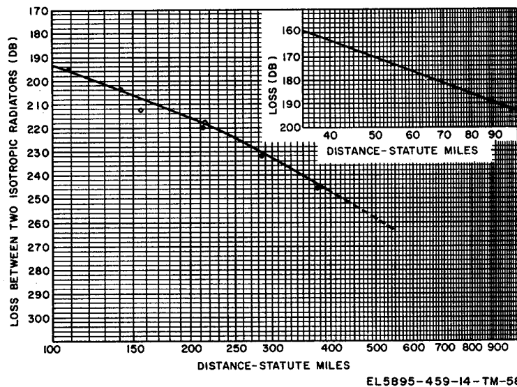
Figure 6-9. Free space attenuation at 1,000 MHz.
