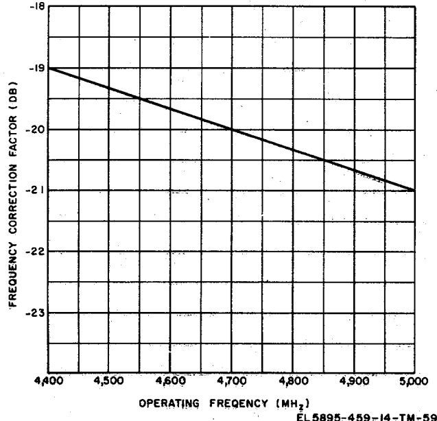
Figure 6-10. Correction table for free space attenuation at frequencies between 4.4 and 5.0 GHz.
