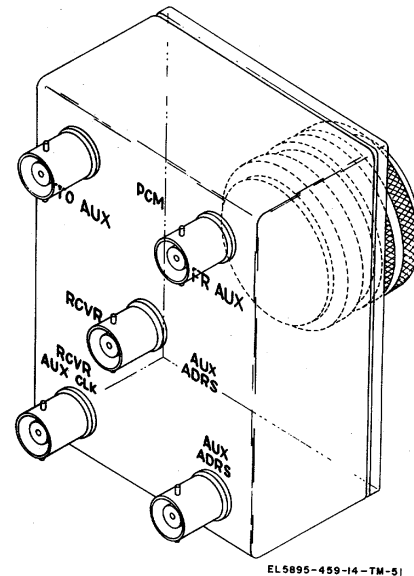
Figure 3-5. Adapter Connector UG-1923/G
