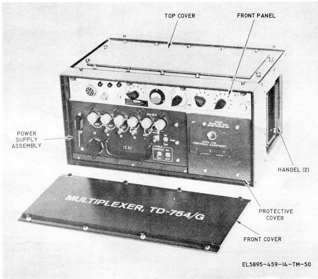
Figure 3-2. Multiplexer TD-7541G.
